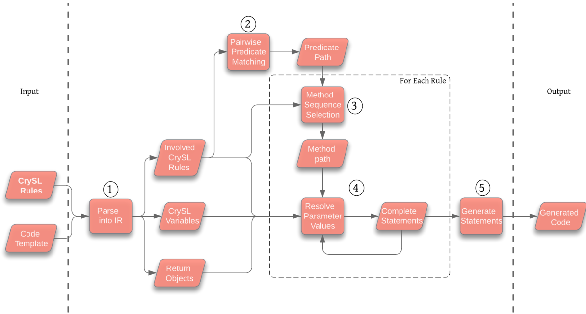
Figure 6. The General Workflow of \text{COGNICRYPT}_{\text{GEN}} .
